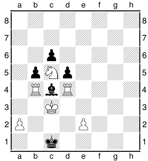
8 (Matt in 3)
