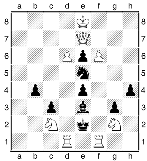
22 (Matt in 3)
