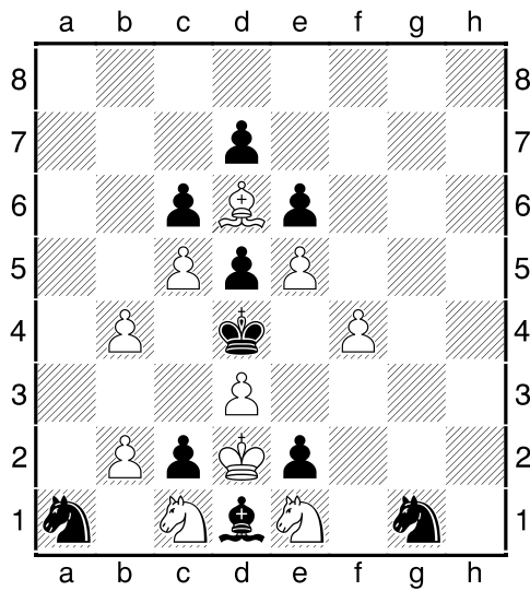
3 (Matt in 2)
