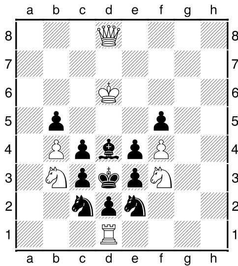
11 (Matt n 2)
