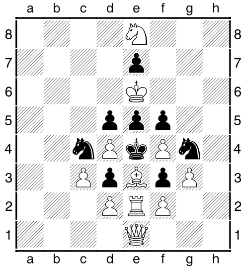
13 (Matt in 3)
