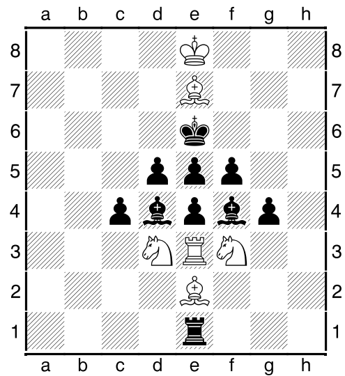
12 (Matt in 3)
