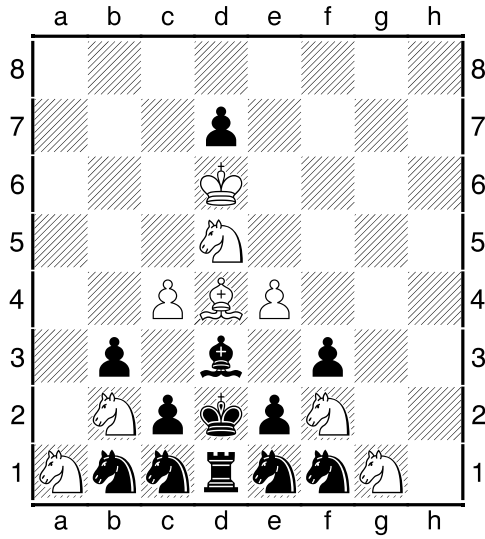
1 (Matt in 2)
