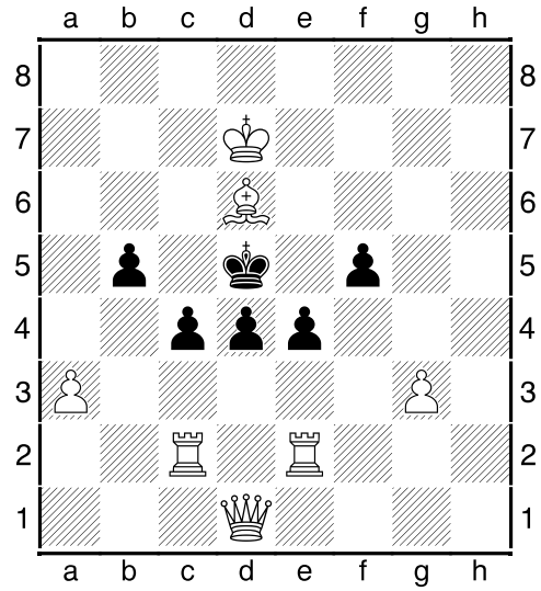
2 (Matt in 2)
