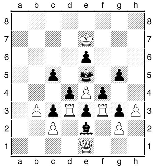
14 (Matt in 3)
