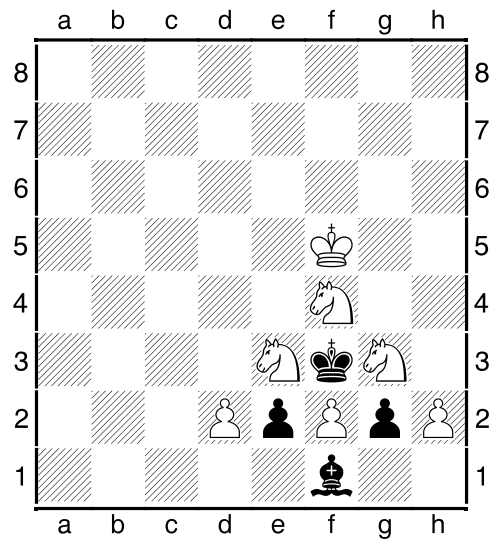
18 (Matt in 3)
