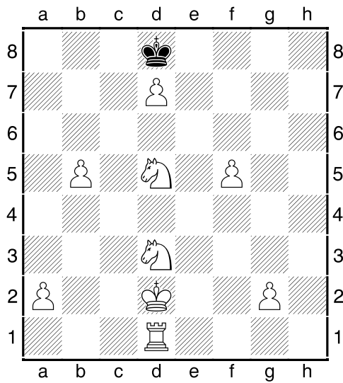
15 (Matt in 3)
