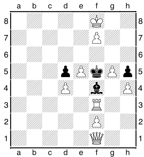
6 (Matt in 2)
