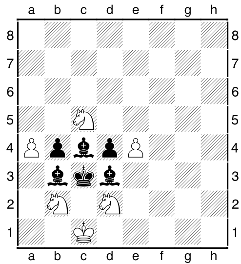
16 (Matt in 3)
