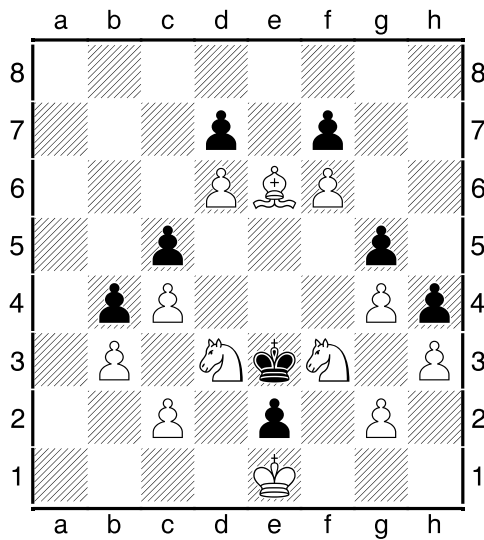
23 (Matt in 4)
