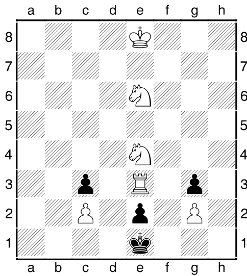
21 (Matt in 5)
