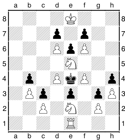
17 (Matt in 5)
