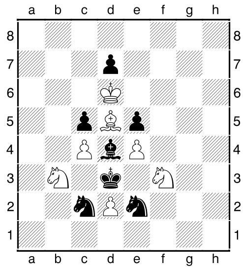
4 (Matt in 2)
