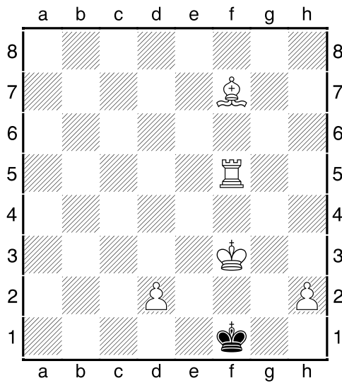
9 (Matt in 3)
