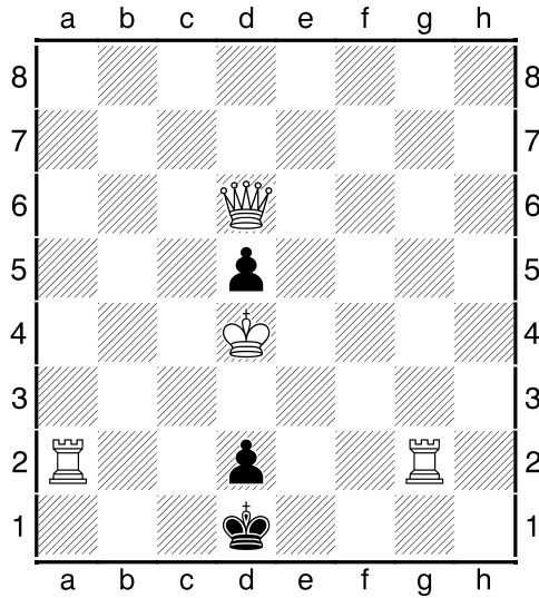
7 (Matt in 2)
