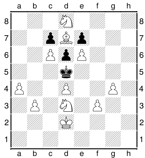
24 (Matt in 5)
