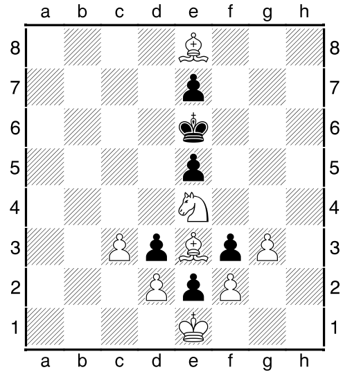
20 (Matt in 5)
