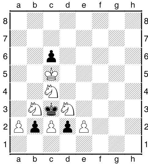
19 (Matt in 4)
